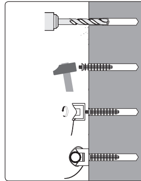
Installation with ELEFIX M7 anchor
